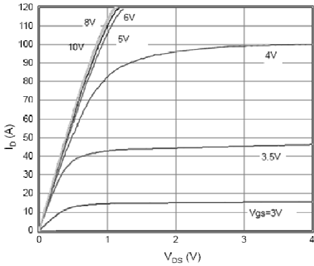
Output Characteristic
