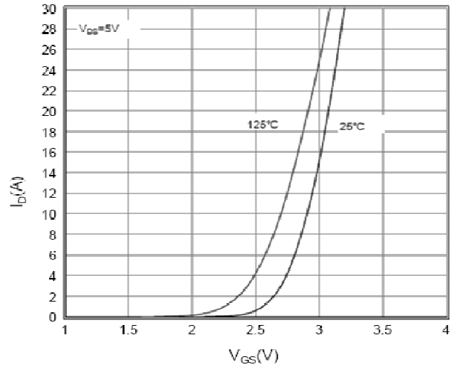
Transfer Characteristic
