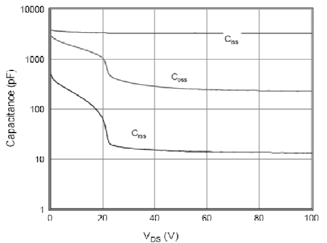
Capacitance
