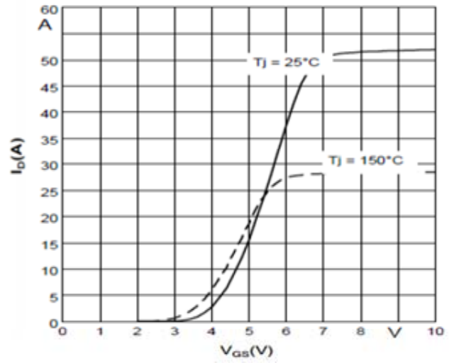
Transfer Characteristic
