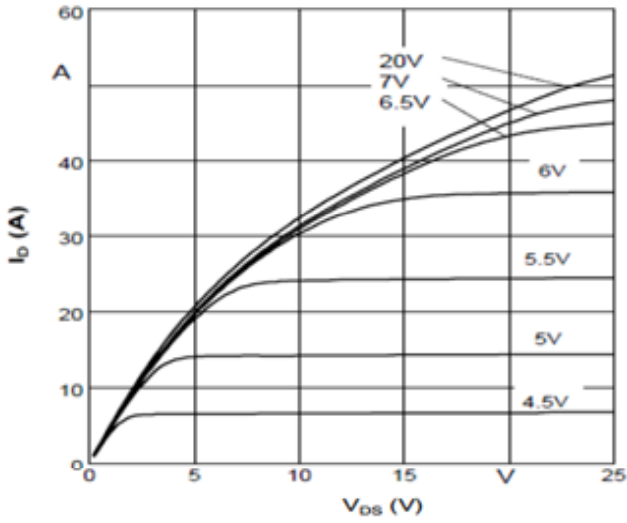
Output Characteristic
